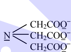
Nitrilotriacetate (nta 3- )
