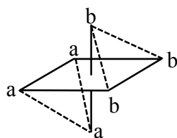
Facial (fac)
