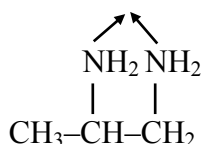
Propylenediamine(pn)
