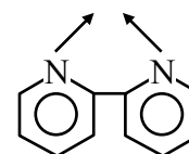
2, 2'-Dipyridyl (Dipy)
