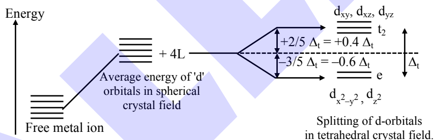
Figure showing crystal field splitting in tetrahedral complex.
