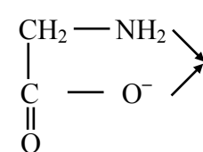
Glycinate (Gly -1 )
