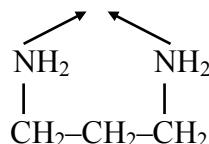
Trimethylenediamine(tn)
