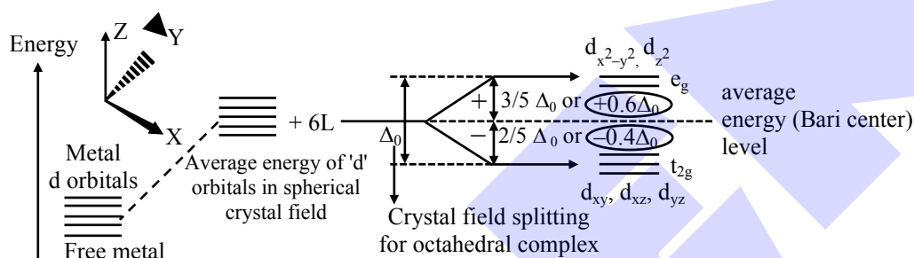
Figure showing crystal field splitting in octahedral complex.
