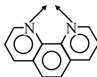
1,10-Phenanthroline (O-phen)
