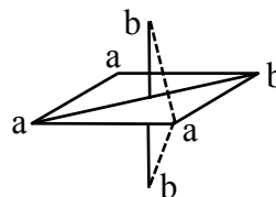
Meridional (Mer)
